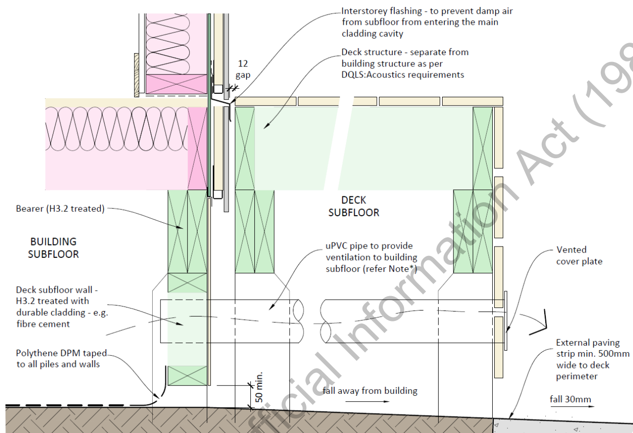
Figure 7-1 Sub-floor Wall between Deck and Building
