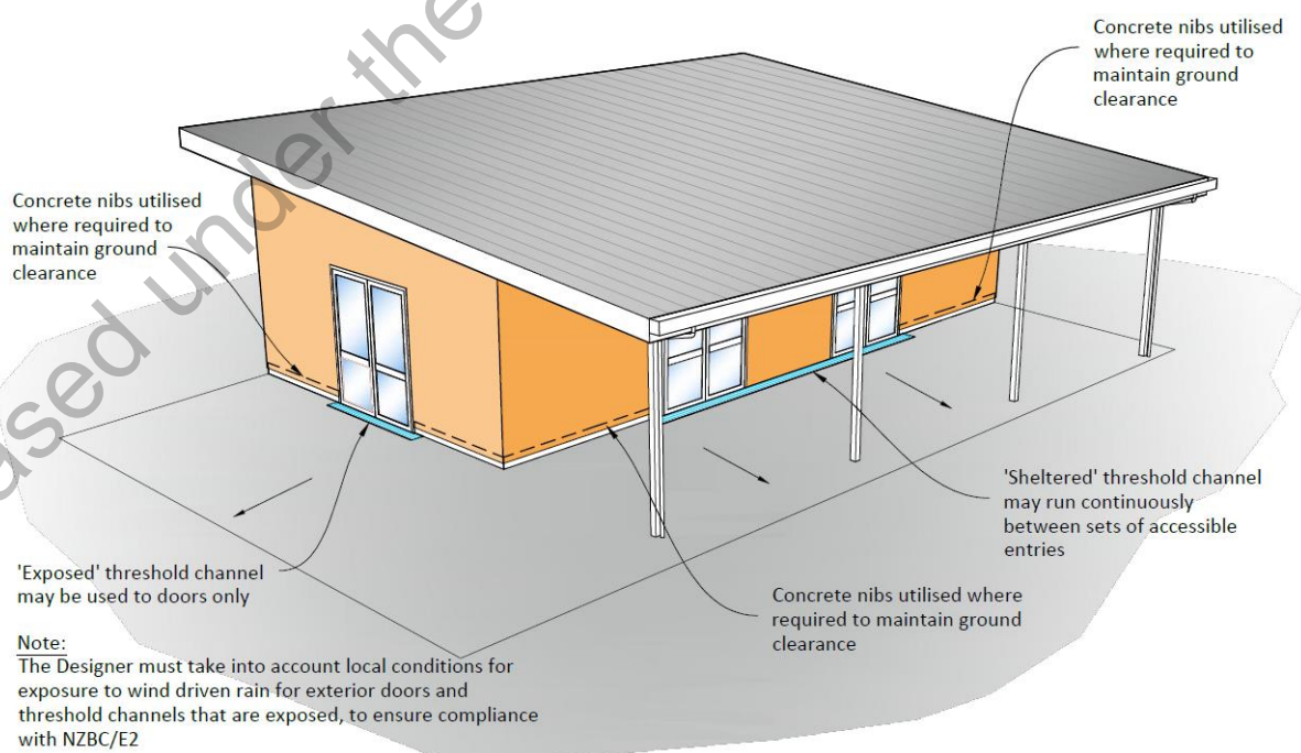
Figure 6-2 Example of Sheltered and Exposed Threshold Channels
