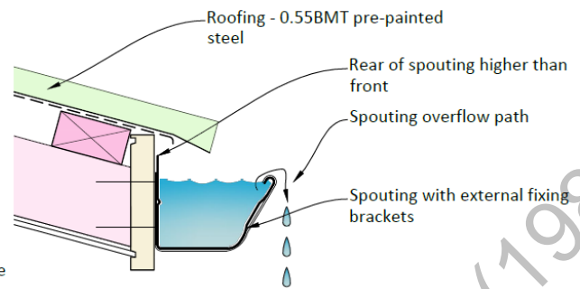
Option 2 - Front overflow
