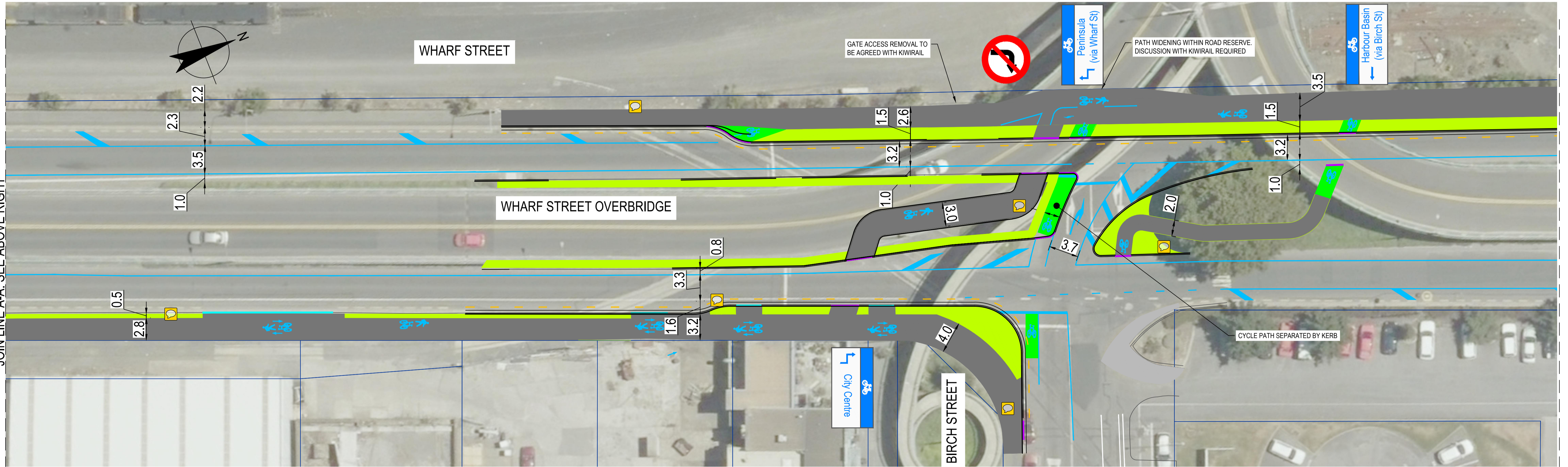
PLAN SCALE 1:250 (A1)
