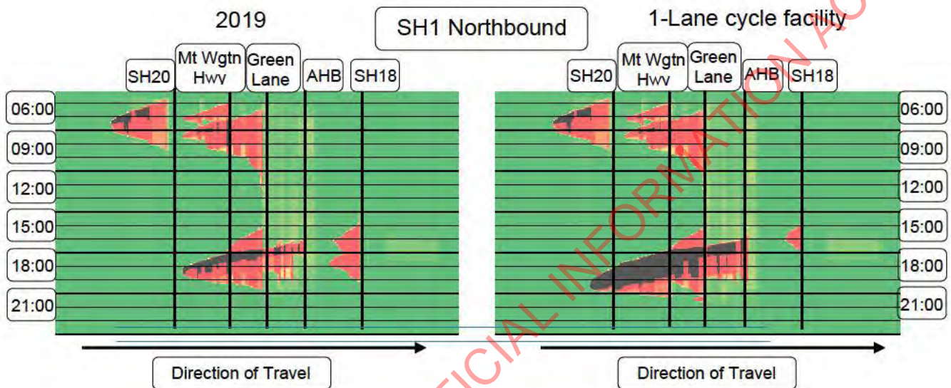
Figure 23 – Option 3a – Impact of example incident scenario on network resilience
