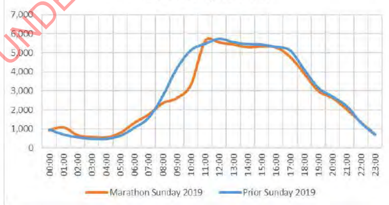
Figure 12 - Auckland Marathon 2019 Traffic Impacts - SH1 SB
