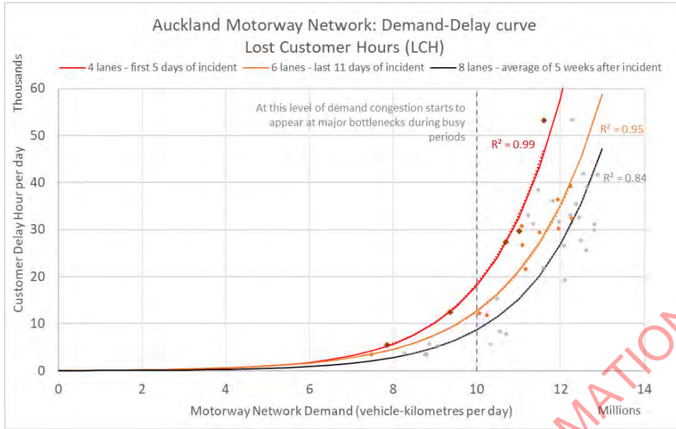
Figure 17 – Effect of lane closures in response to Sept-20 bridge strike on motorway network capacity
