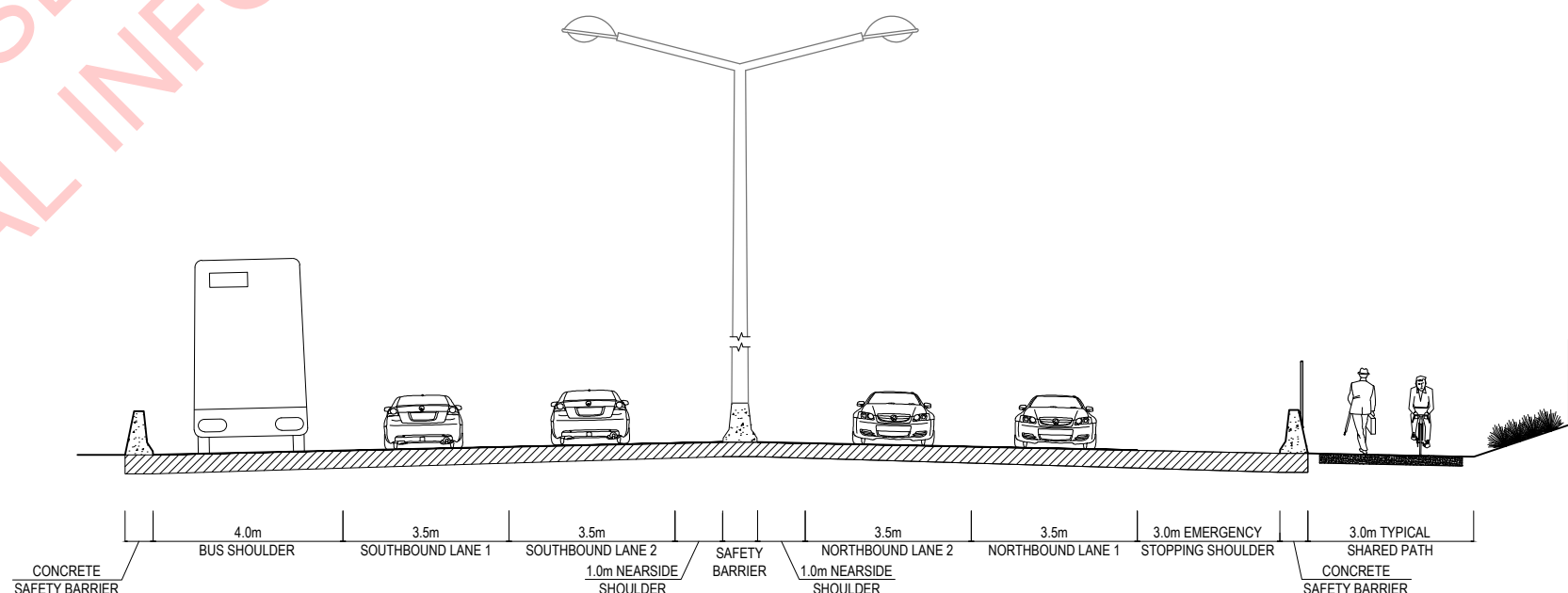
1 TYPICAL CROSS SECTION SCALE 1:75
