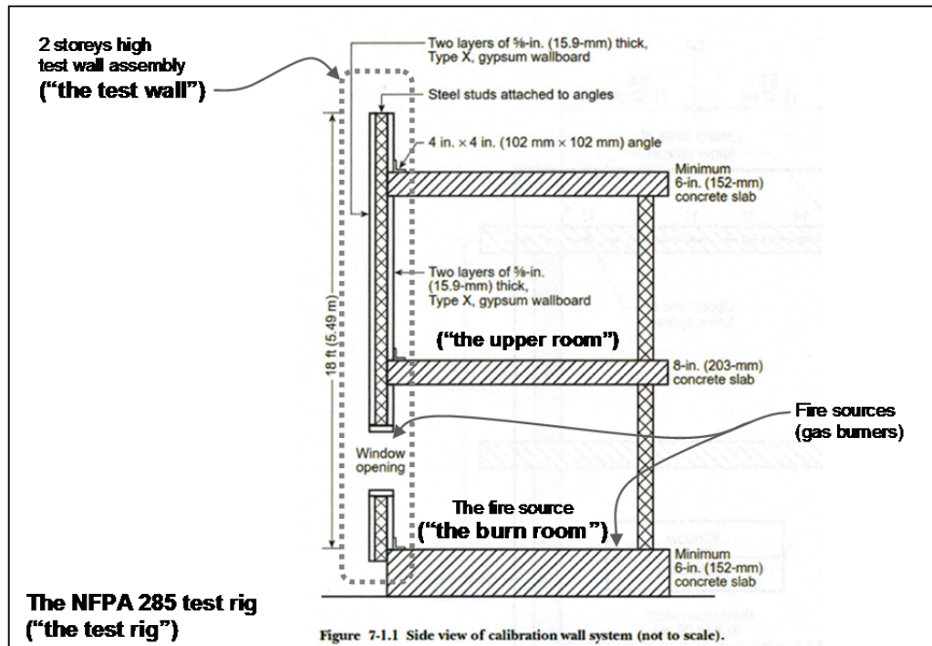
Figure 3: The NFPA 285 fire test rig 16
