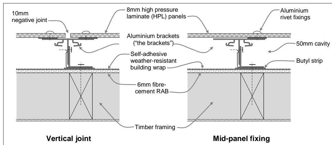
Figure 1: Typical construction of the original façade system (not to scale)
