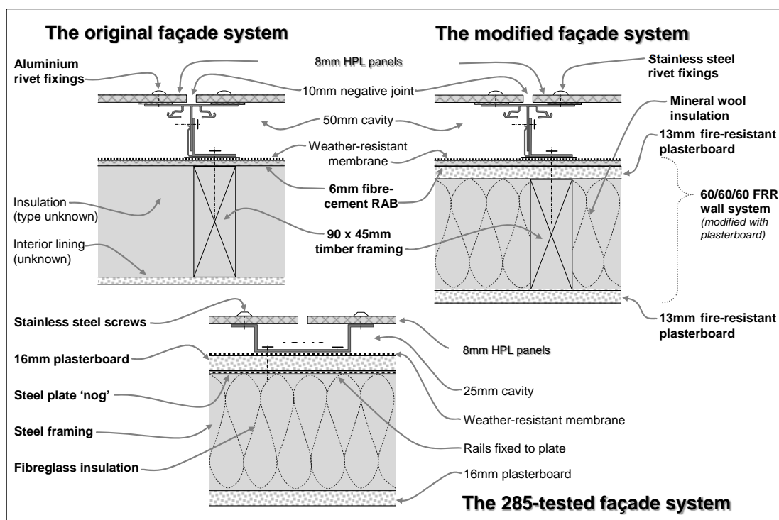
Figure 2: The original, modified, and 285-tested façade systems (not to scale)
